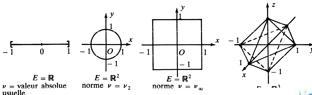
Fig. 1. Boule \tilde{\mathbf{B}}(0_E, 1) .
