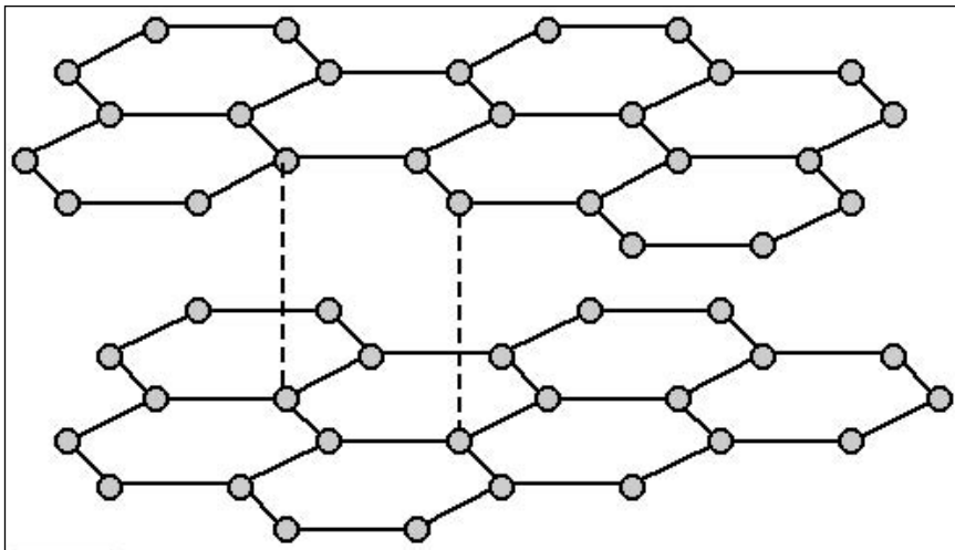
Figure 3.2 Structure du graphite
